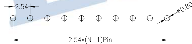
Recommended P.C.B Layout(Top Side) (PCB BOARD TOLERANCE±0.05)
